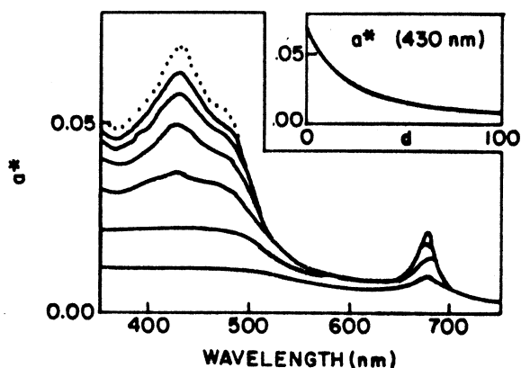
Fig. 3 _ Change in spectral values of the specific absorption coefficient a^* (in m^{-1} (mg \text{ chl } a \text{ } m^{-3})^{-1} ) for algal cells containing the same material but differing size (diameter, d , in \mu m ). The dotted curve represents the spectral absorption values of this material (arbitrarily chosen) as dispersed in solution ( d \rightarrow 0 ). The continuous curves, from the upper to the lower one, correspond respectively to the diameters 2, 4, 8, 16, 32 and 64 \mu m . Inset: variations with the cell diameter of the specific absolute value of absorption at 430 nm. In: Bricaud and Sathyendranath (1981), p.46.
