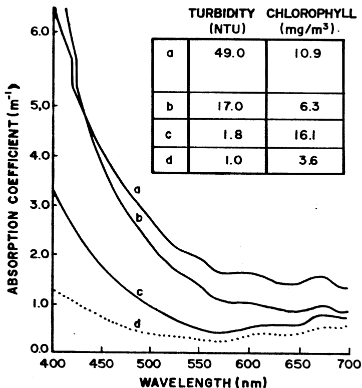
Fig. 5 _ Total absorption spectra of various natural waters in southeastern Australia. The values of turbidity (NTU) and total chlorophyll content (mg m -3 ) for each curve are listed beside. Adapted from Kirk (1983), p.65.
