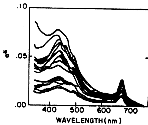
Fig. 2 _ Spectral values of specific absorption, a^* (expressed in m^{-1} (mg (chl a + pheo a) m^{-3})^{-1} ) determined on intact cells during exponential growth, for different algal species in batch cultures. In: Bricaud and Sathyendranath (1981), p.45.
