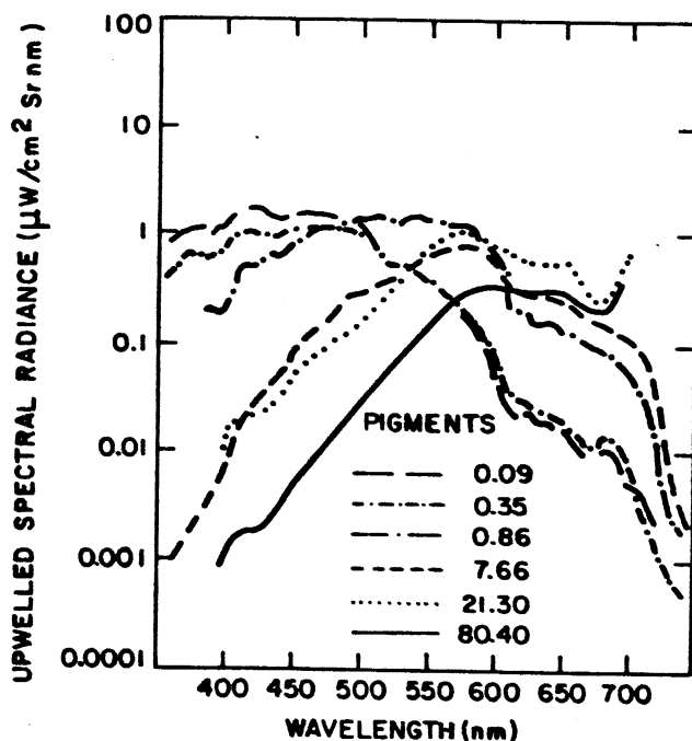
Fig. 4 _ Upwelled spectral radiance as a function of chlorophyll pigment concentration for various ocean waters. In: NASA (1987), p. 14.
