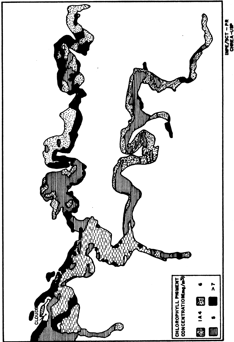
Fig. 6 - Chlorophyll pigment distribution in Barra Bonita Reservoir
