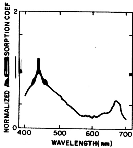
Fig. 1 _ Absorption curve (normalized at 440 nm) of phytoplankton and covarying detrital matter. Obtained in the study of Prieur and Sathyendranath apud Bricaud and Sathyendranath (1981), p.44.
